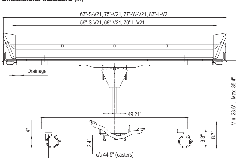
Comes with four, 4 in. (100 mm) braked twin castors as standard. Straight steering option available.
