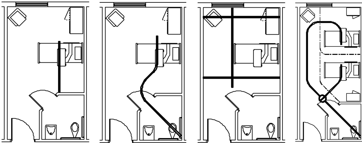
TRACK LAYOUTS These are just a few of the many track layout options available for specific needs including curves, turntables, door pass through and XY axis configurations.
